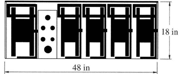
Front View of Cabinet
