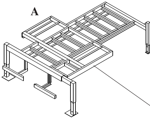
Crane base ties directly into body substructure
